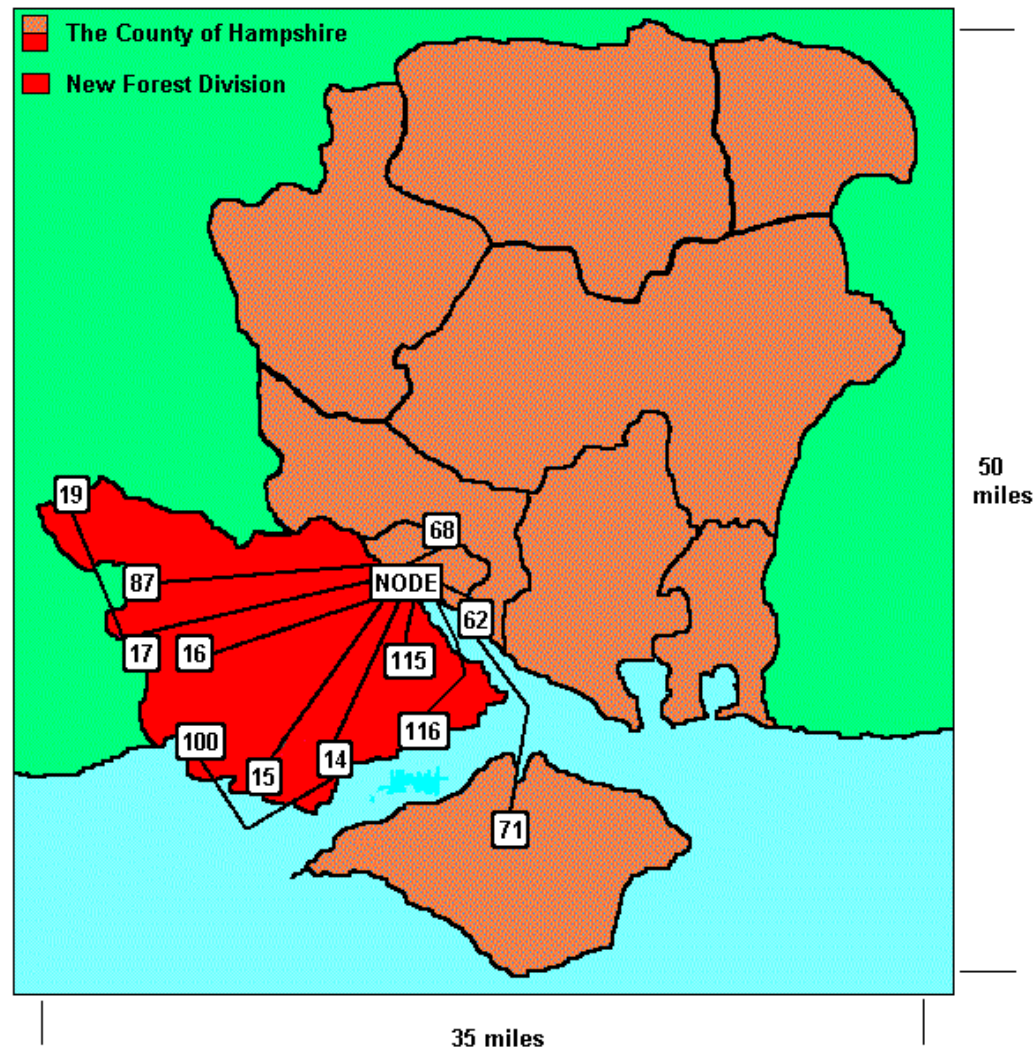
Hampshire Constabulary - New Forest Division - QS UHF Scheme
